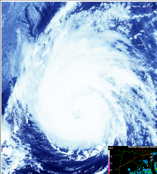
Visible Cloud Imagery (GOES-East)
