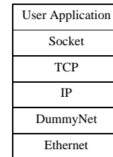
Figure 3: WASP Approach
