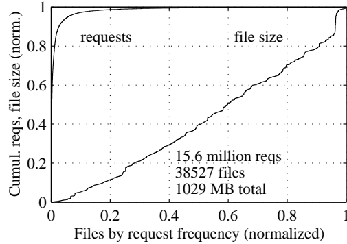
Figure 6: IBM Trace
