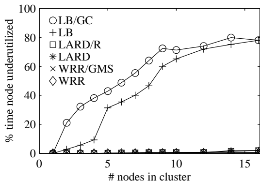
Figure 9: Idle Time
