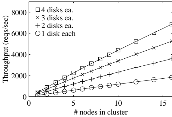
Figure 13: WRR vs disks
