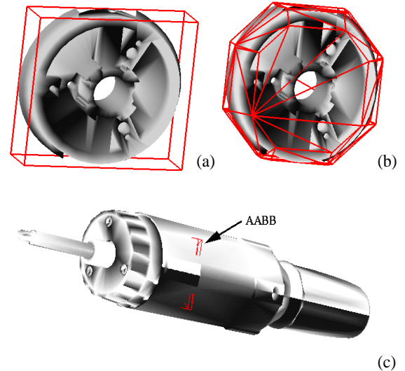
Figure 1: Servo screwdriver: (a) motor part and AABB; (b) motor part and 26-dop; (c) AABB of motor part is visible through hull, while 26-dop is completely occluded by hull.
