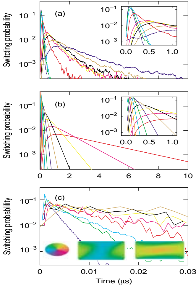
FIG. 1. Fig. 1: (a) Measured switching probability vs. time, for one sample at 300 K, for a number of different values of H_C - H between 1 and 6 Oe. Inset is a blowup of the same data near t=0 . (b) Predicted switching probability vs. time from the energy-ladder model for N=4 , q=0.001 , and for a range of p values. (c) Predicted switching probability vs. time from the micromagnetic simulation of a rectangular sample at 300 K, averaged over 1000 switching events. Insets show the magnetization direction in the sample for a typical run before (left panel) and after (right panel) the switch.
