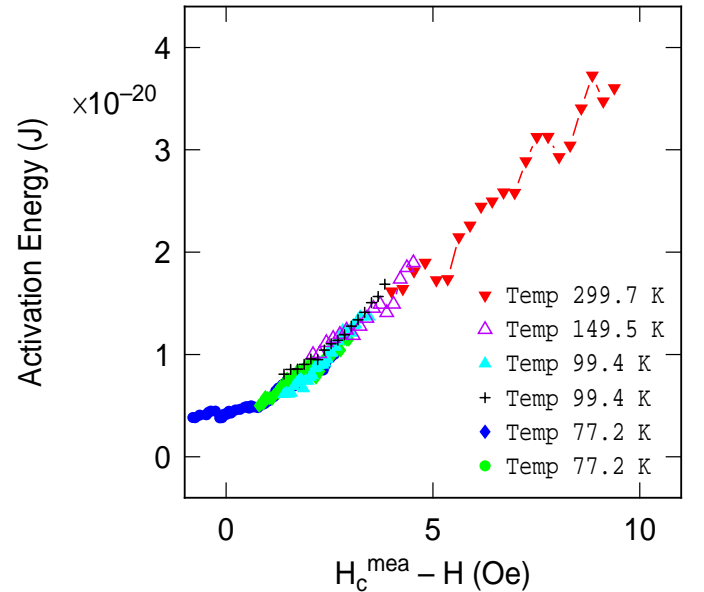
FIG. 2. Fig. 2: Measured activation energy vs. H_C - H for four temperatures and two samples.
