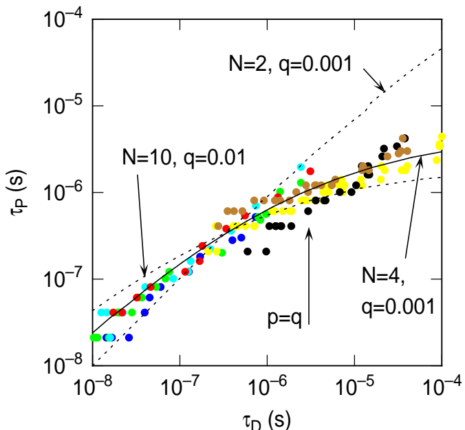
FIG. 3. Fig. 3: Measured values of \tau_P vs. \tau_D for 7 samples at 300 K. The solid and dashed lines are predictions from the energy-ladder model for the indicated values of N and q .
