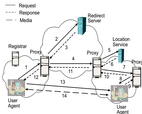
Fig. 1. SIP architecture
