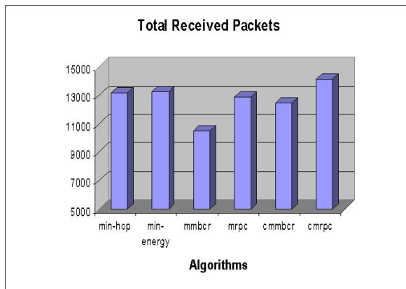
Fig. 6. Total Packet Throughput (UDP Sources), R=1.5
