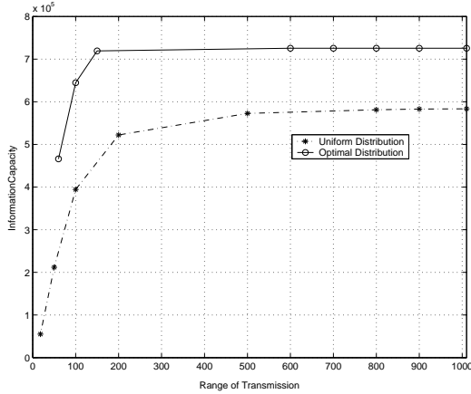
Figure 8: Data delivered vs. limit of transmission range
