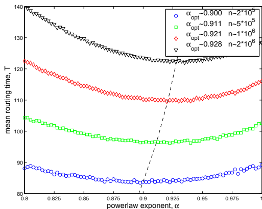
FIG. 3: Mean routing time T(\alpha) for several network sizes. The dashed line shows the path \alpha_{\text{opt}} , defined as the minimum of the best quadratic fit, follows as n increases.
