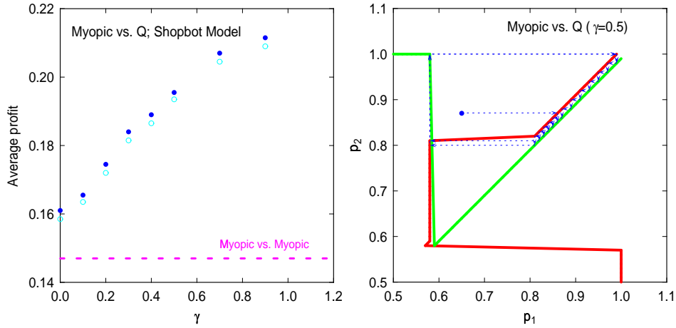
Fig. 2. Results of single-agent Q-learning in the Shopbot model. (a) Average profit per time step for Q-learner (seller 1, filled circles) and myopic seller (seller 2, open circles) vs. discount parameter \gamma . Dashed line indicates baseline expected profit when both sellers are myopic. (b) Cross-plot of Q-derived price curve (seller 1) vs. myopic price curve (seller 2) at \gamma = 0.5 . Dashed line and arrows indicate a temporal price-pair trajectory using these policies, starting from filled circle.
