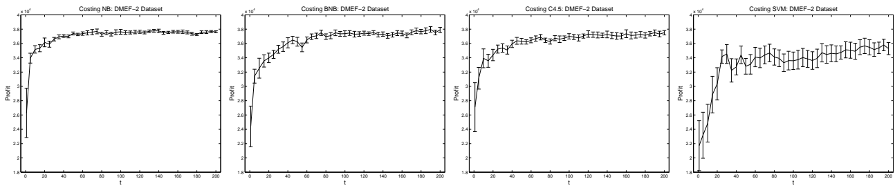
Figure 2. Costing: test set profit vs. number of sampled sets.
