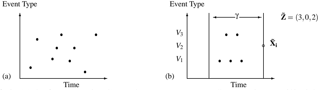
Fig. 1: (a) A plot of event type vs time. (b) For each target event X_i , we capture all events previous to X_i within window size \gamma . The result is a count vector indicating the number of instances for each event type.
