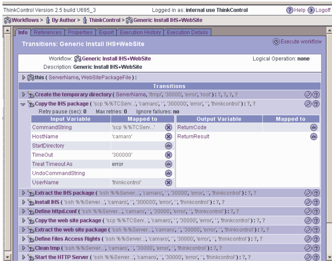
Figure 1: Steps for Provisioning an http Server from a Service Provisioning System
