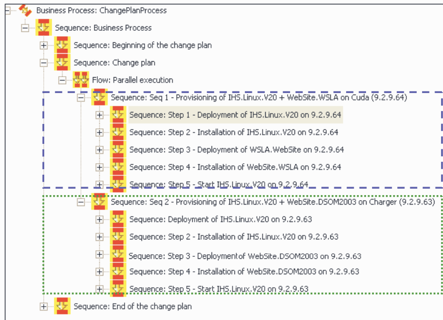
Figure 4: Concurrent Provisioning of 2 Websites
