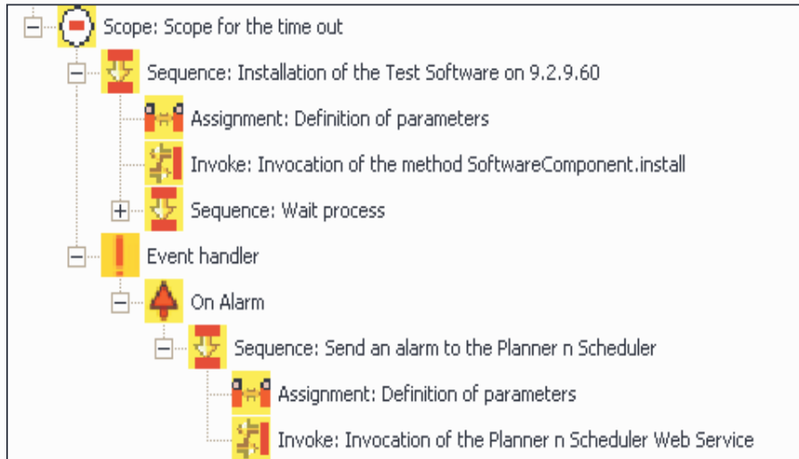
Figure 6: Enforcing Deadlines and Durations
