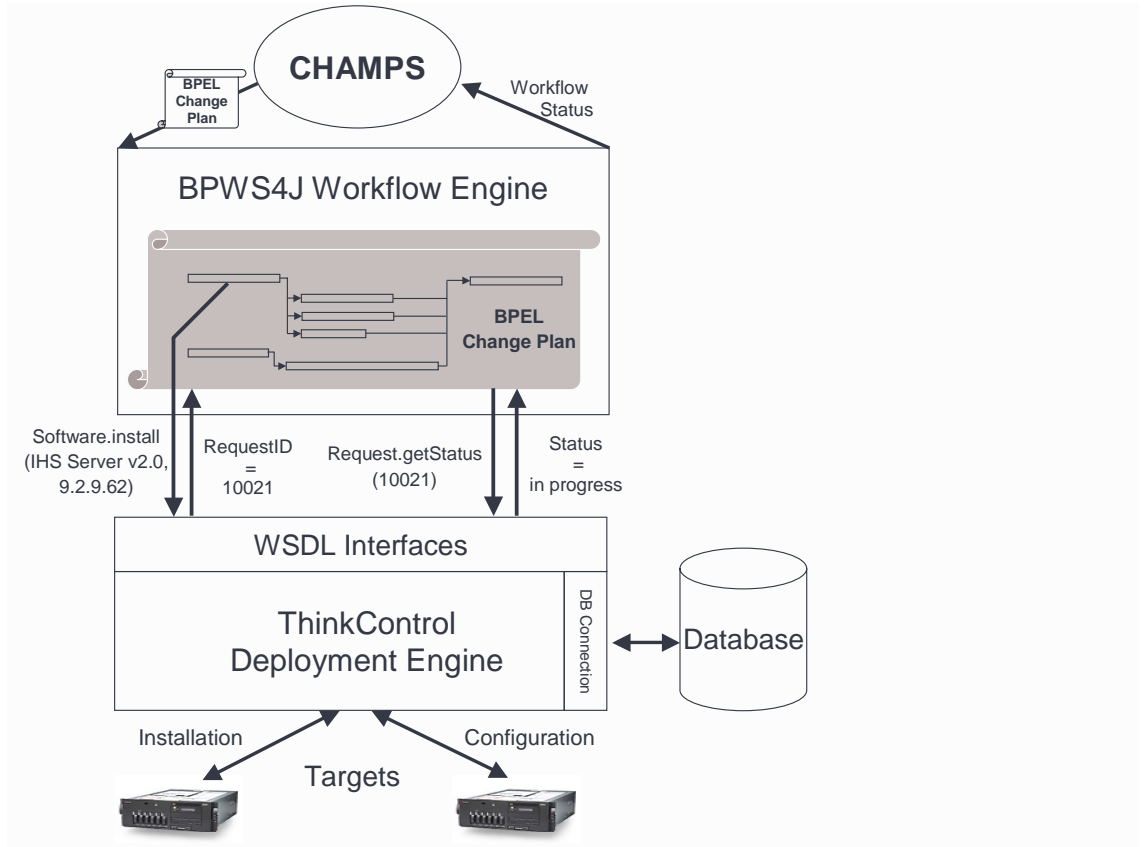
Figure 3: Prototype for integrating the TIO Provisioning System with the CHAMPS Change Manager
