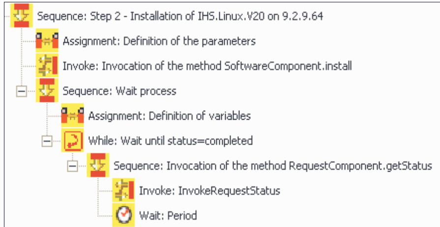
Figure 5: Monitoring Task Execution Status
