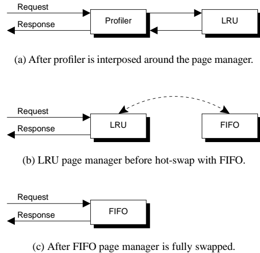
Figure 1: Online reconfiguration. This figure shows two online reconfiguration mechanisms: interposition and hot-swapping. (a) shows an LRU page manager and an interposed profiler that can watch the component's calls/returns to see how it is performing. If it determines that performance is poor, it may decide to switch the existing component for another. (b) shows the LRU page manager as it is about to be swapped with a FIFO page manager. Once the swap is complete, as shown in (c), the LRU page manager can be deleted.
