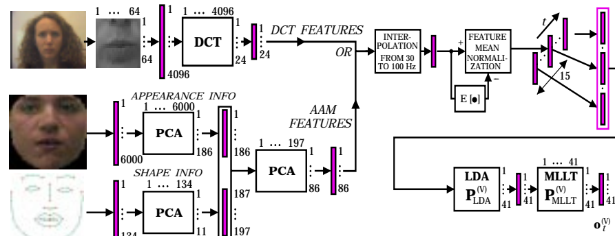
Figure 1: DCT versus AAM based visual feature extraction for automatic speechreading, followed by linear interpolation, feature mean normalization, and the application of LDA and MLLT.
