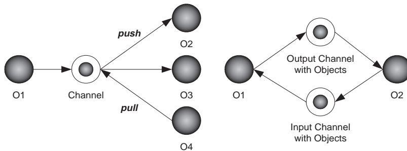
Fig. 4. Channel-based Messaging
