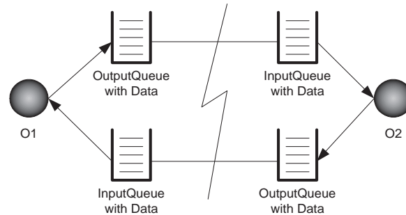
Fig. 5. Queue-based Messaging
