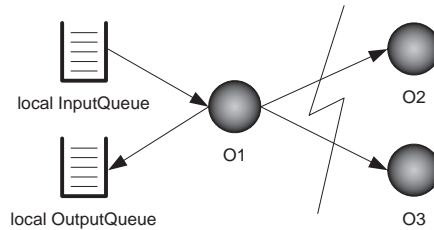
Fig. 6. MQ-Integrating Transactions
