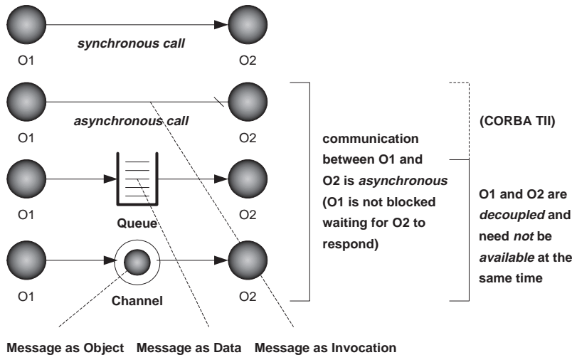
Fig. 2. Event Notification
